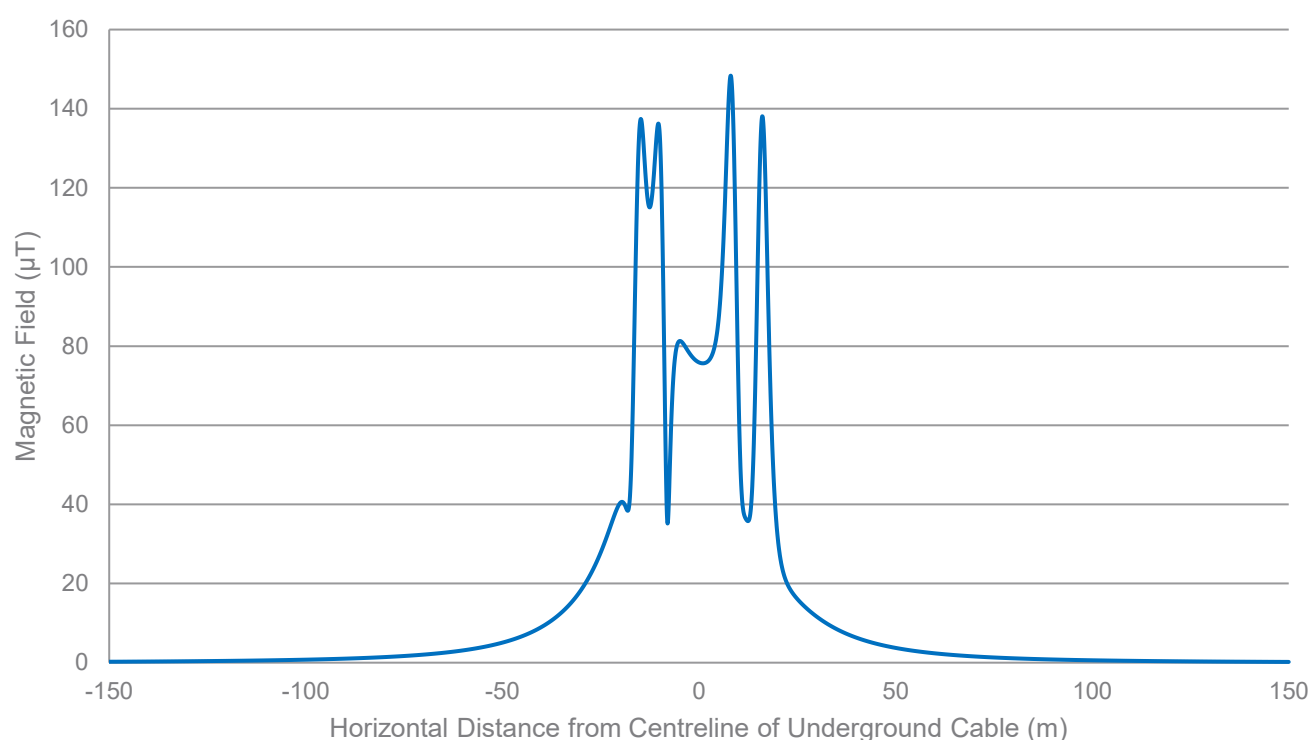
Figure 6.7 Combining Magnetic Fields from Underground Cables in Close Proximity to New Overhead Lines for Two Cables Per Phase
