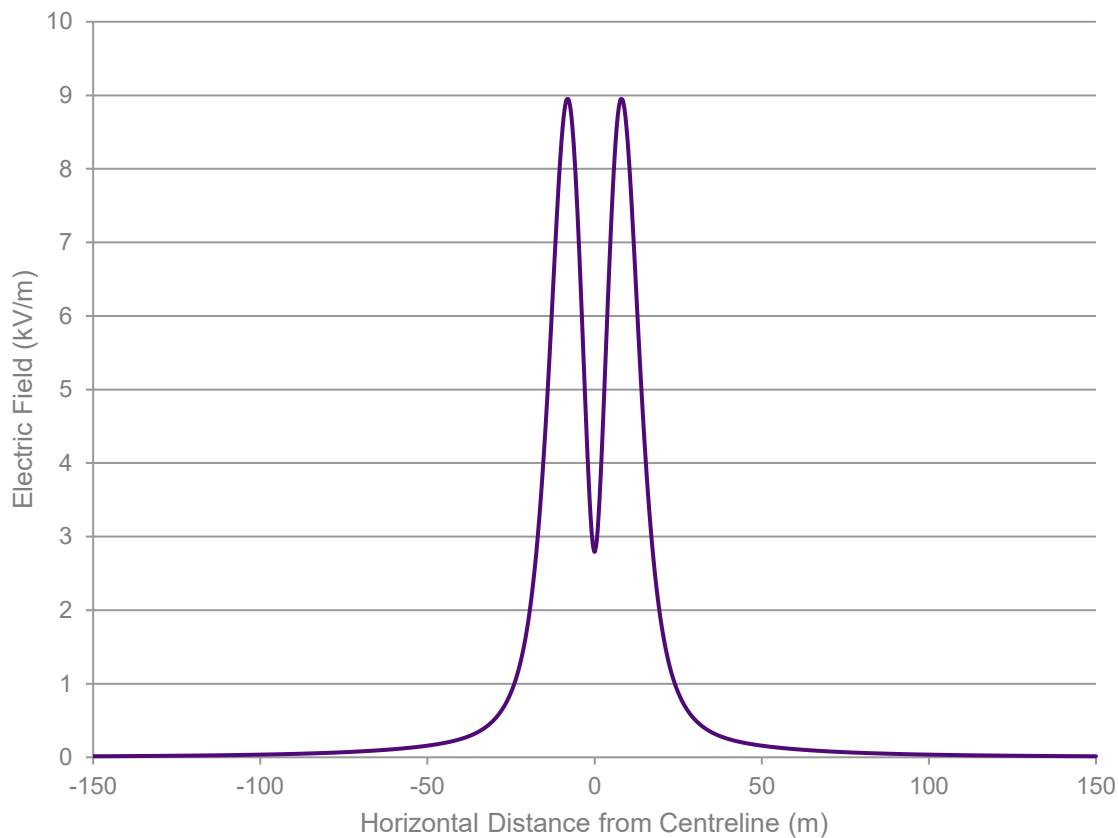
Figure 6.1 Maximum Electric Fields from the New 400 kV Overhead Line
