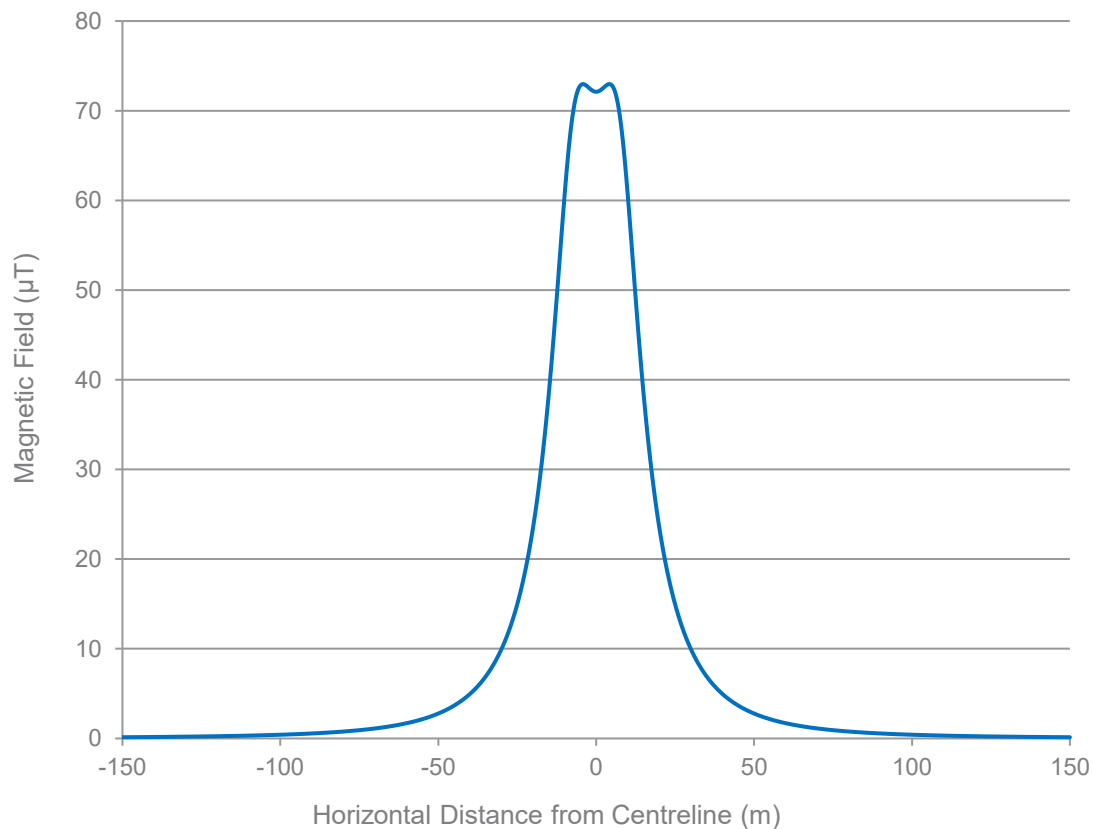
Figure 6.2 Maximum Magnetic Fields from the New 400 kV Overhead Line
