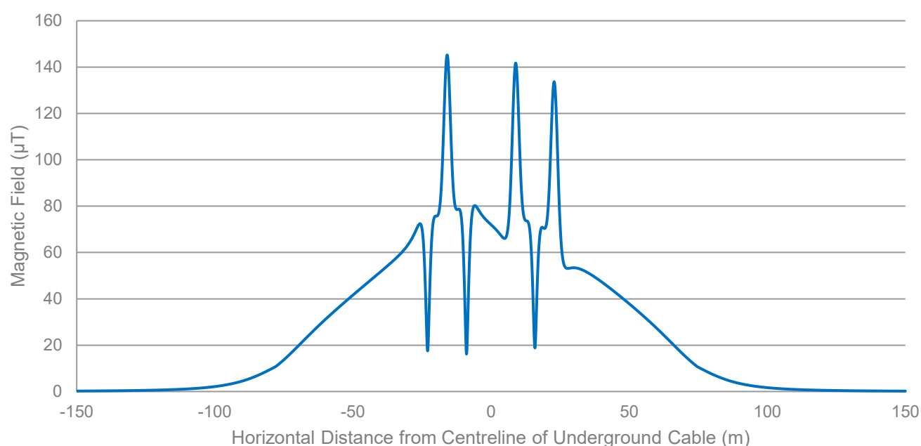
Figure 6.8 Combining Magnetic Fields from Underground Cables in Close Proximity to Existing Overhead Lines for Three Cables Per Phase
